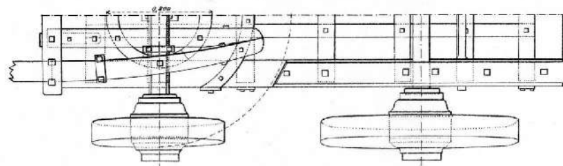
Fig.2 Plan horizontal
